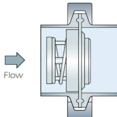
Installed valve
